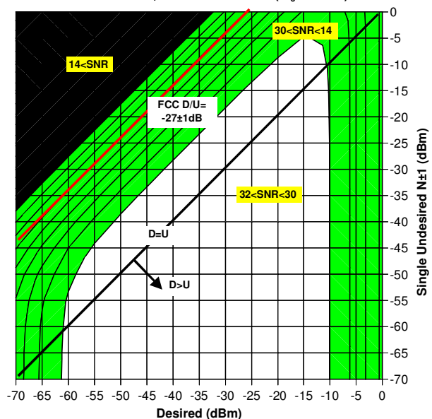
Figure 1b: Receiver Post-decoder SNR Conours (2dB interval) Tx SNR=32dB ; Excellent Receiver ( IP_3=32\text{dBm} )
