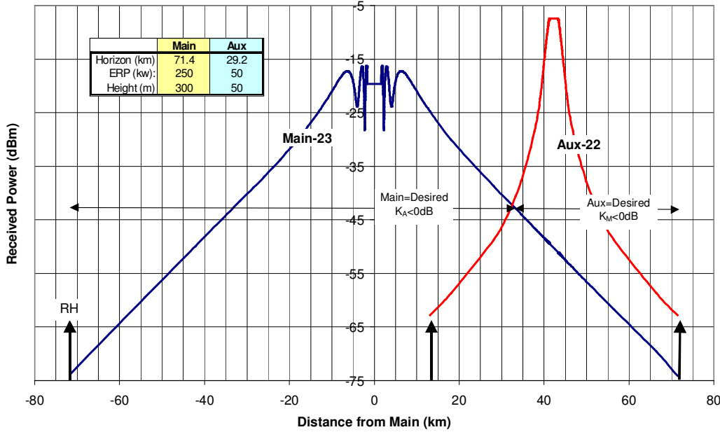
Figure A4: Received Power of Main Channel 23 and Auxiliary Channel 22 F(50,90) ; Rx Antenna gain at Tuner=6dBd
