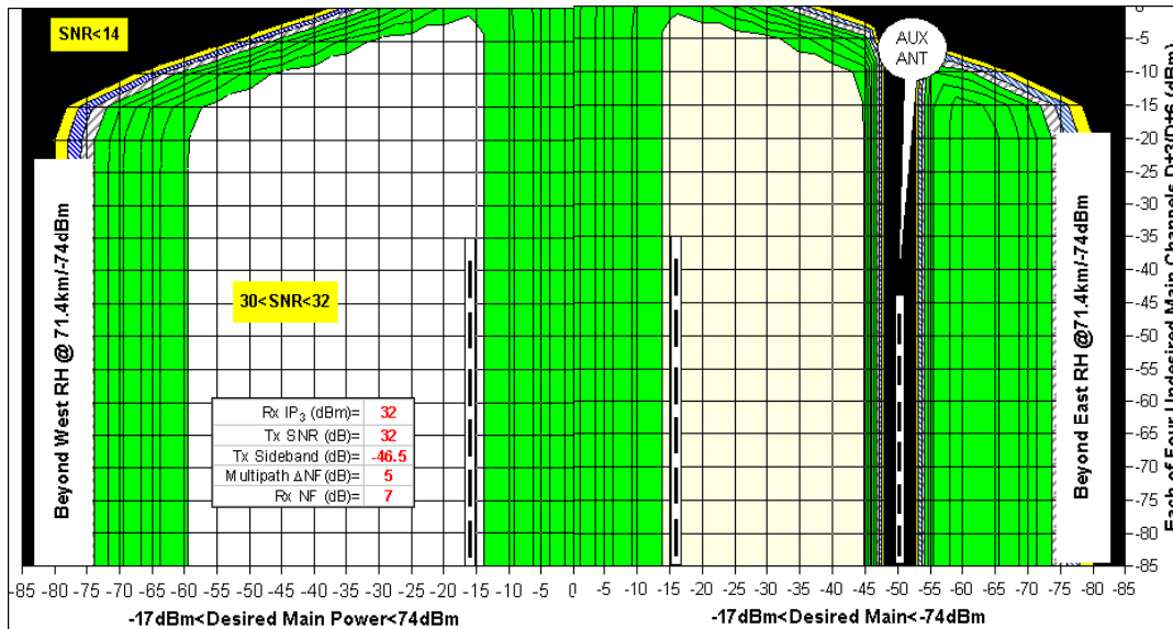
Figure 7: Post-decoder SNR Contours (2dB intervals) of Main-23 F(50,90) ; Rx Antenna @ 30feet AG ; Rx IP_3=32 dBm
