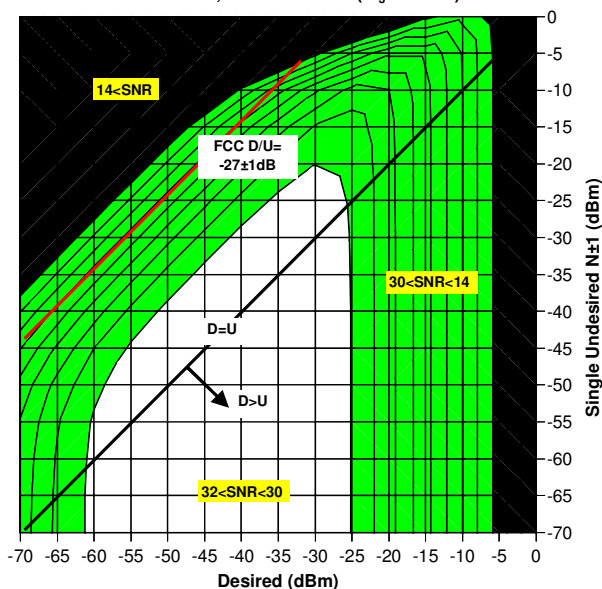
Figure 1a: Receiver Post-decoder SNR Conours (2dB interval) Tx SNR=32dB ; Good Receiver ( IP_3=16\text{dBm} )
