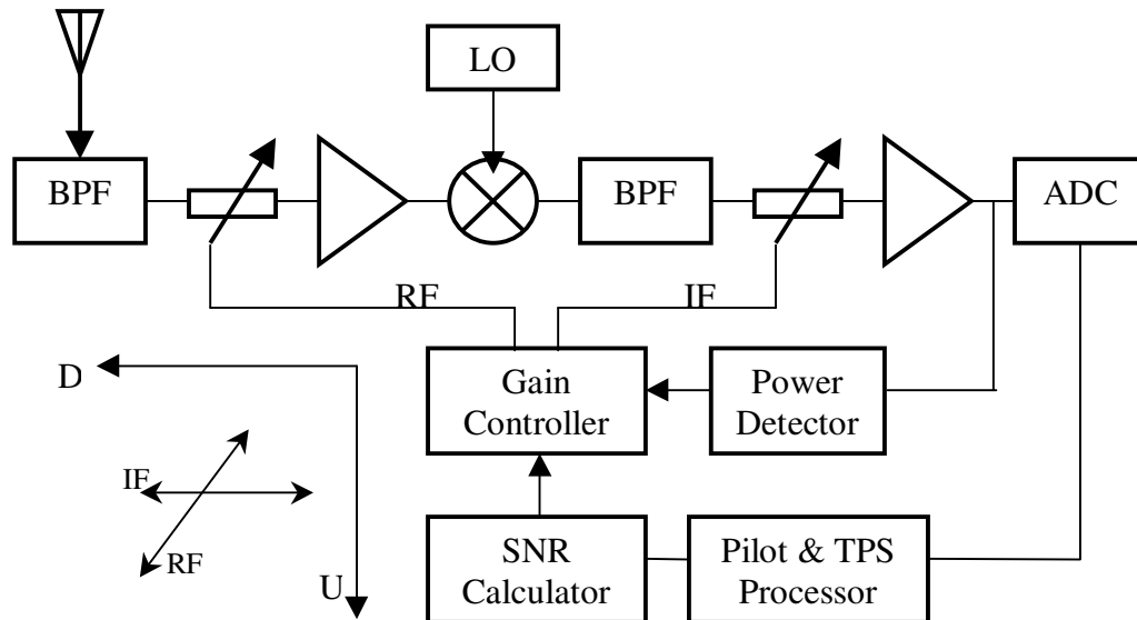
Figure 2: Modified AGC for Adjacent Channel Reception Optimization
