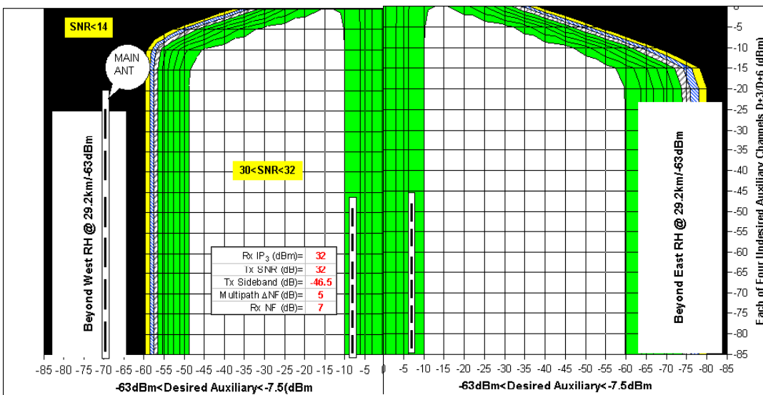
Figure 8: Post-decoder SNR Contours (2dB intervals) of Auxiliary-22 F(50,90) ; Rx Antenna @ 30feet AG ; Rx IP_3=32 dBm
