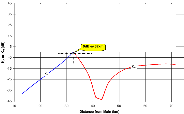
Figure A5: The Factors K_A and K_M
