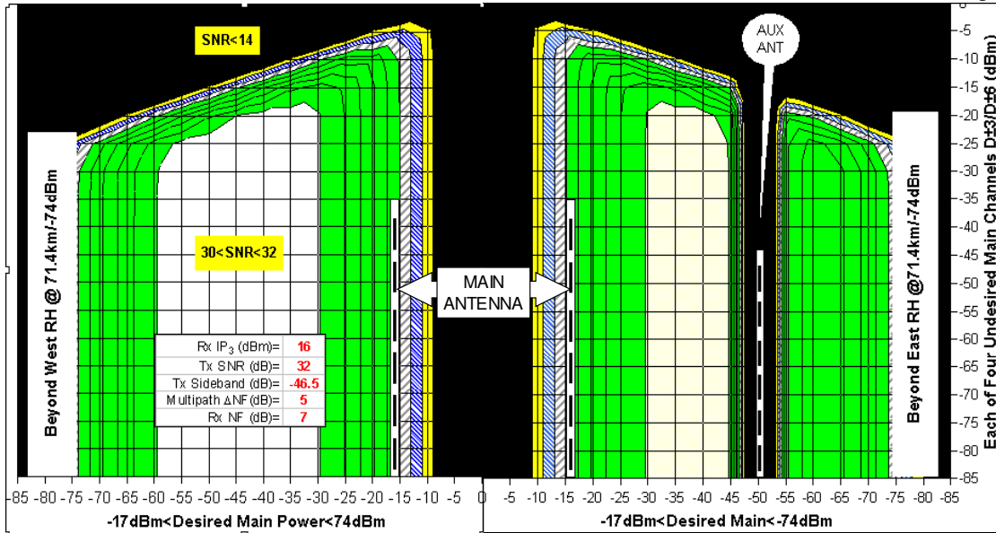
Figure 5: Post-decoder SNR Contours (2dB intervals) of Main-23 F(50,90) ; Rx Antenna @ 30feet AG
