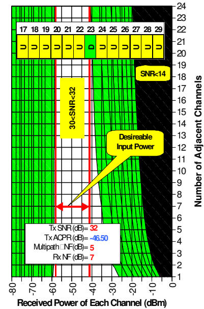
Figure A1: Post-decoder SNR Contours for 1-24 Adjacent, Equal Received Power, Channels 14-37 ; “Good Receiver” ( IP_3=16 )
