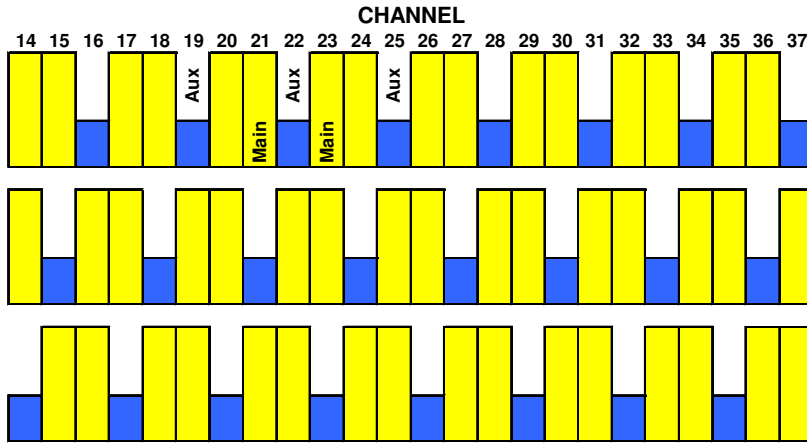
Figure 3: Potential Assignments of 16 Main and 8 Auxiliary Channels in a Market
