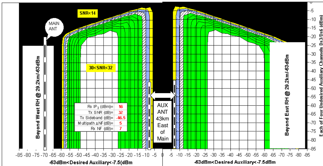
Figure 6: Post-decoder SNR Contours (2dB intervals) of Auxiliary-22 F(50,90) ; Rx Antenna @ 30feet AG
