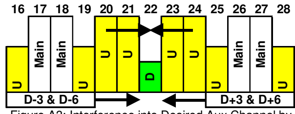
Figure A3: Interference into Desired Aux Channel by Two Pairs of Main Channels and Two Pairs of Aux Channels
