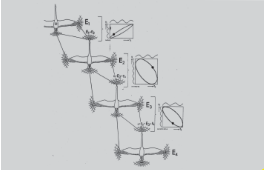
Fig. 28: V-formations can be constructed by means of an equation that I developed on the basis of physical laws. Comparisons with photographs of natural bird formations show that the assumptions are correct: The formations are given by the Coulomb forces between birds that are electrically charged in flight.
