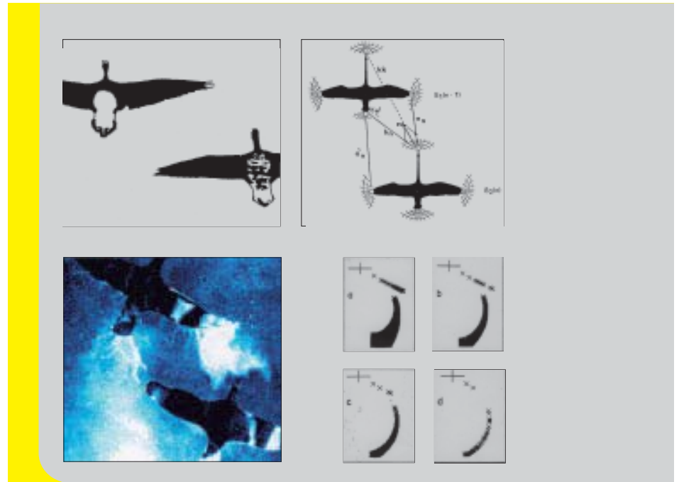
Fig. 27: Birds use electrical fields for formation flying. Top left: Two geese in formation flight. Bottom left: Experimental model to visualise the electrical field forced between these birds. Top right: Vector diagram of the field distribution. Bottom right: Calculation of the position of the bird behind with reducing degrees of freedom a-d. Warnke 1989, Copyright Ulrich Warnke
