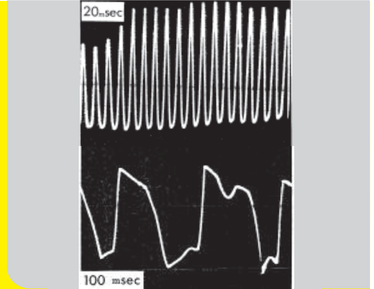
Fig. 14: Oscillogram of the alternating electrical field around bees (top) and pigeons (bottom) in a wind tunnel.
