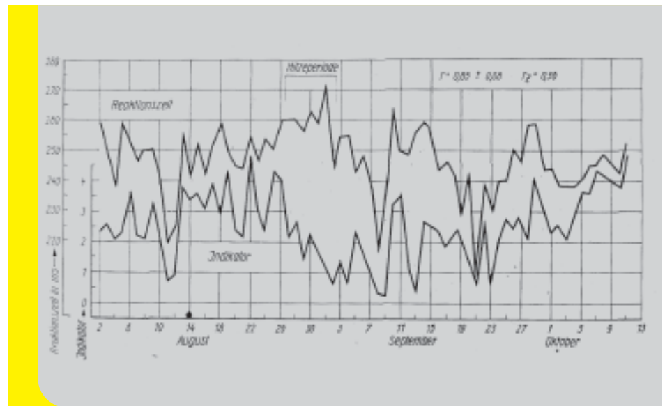
Fig. 5: Significant linear correlation between electromagnetic very long wave activity and average reaction times of exhibition visitors. Reiter, R. 1960 Meteorobiologie und Elektrizität der Atmosphäre. Akademische Verlagsges. Geest & Portig, Leipzig
