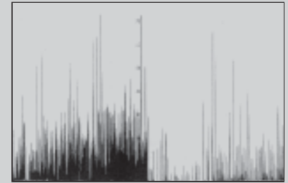
Fig. 1 Top: The "midnight phenomenon". The activity of the electromagnetic impulses (shown on 5 different days) abruptly ends at midnight.
